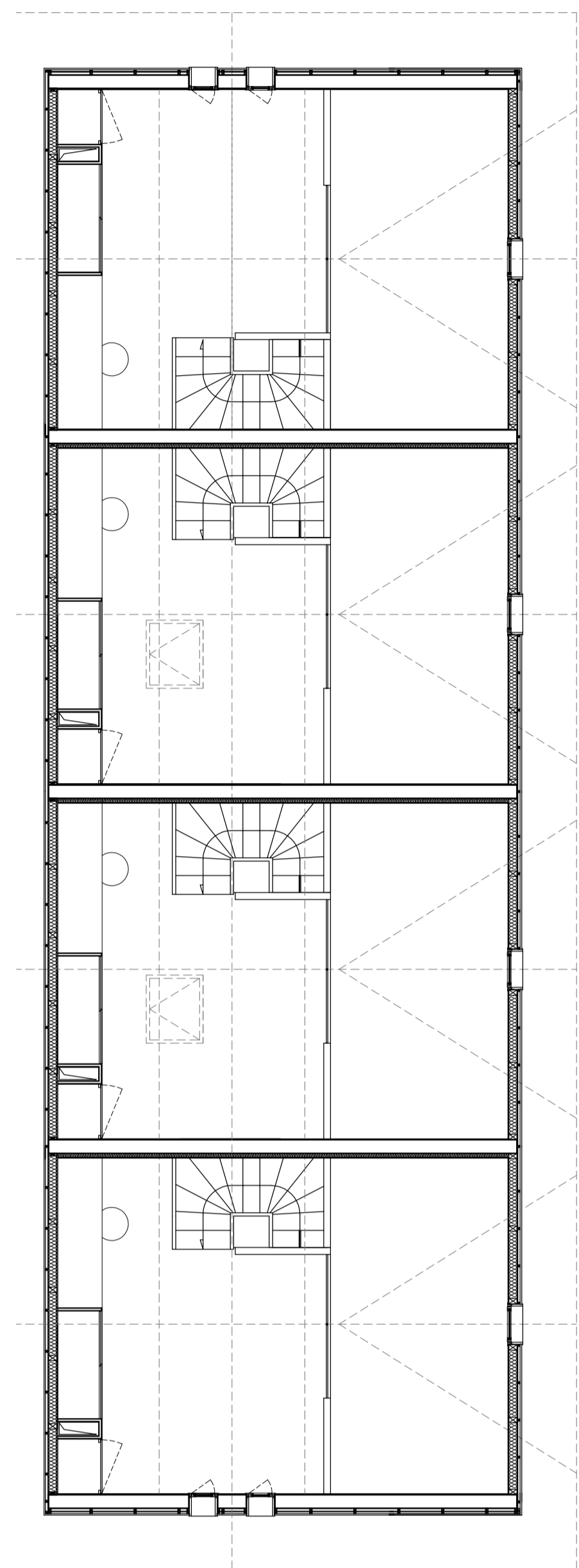
PLAN MEZZANINE
